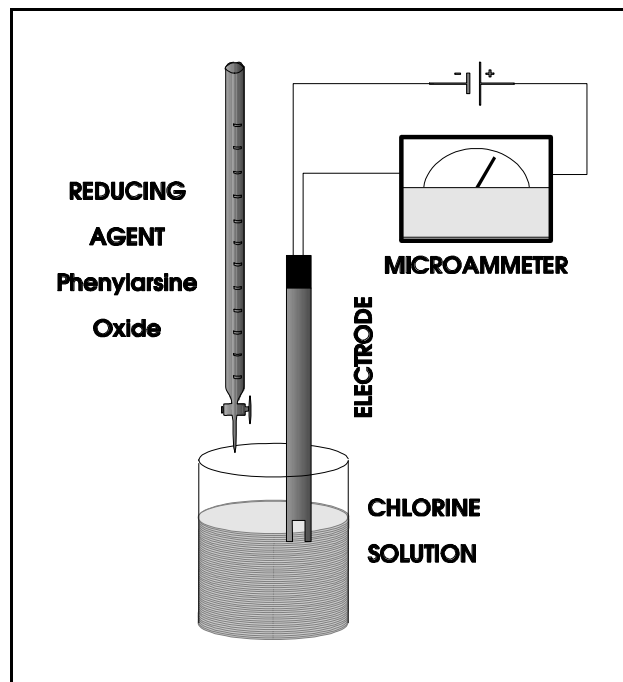
Figure 3 - Amperometric Titration of Chlorine
