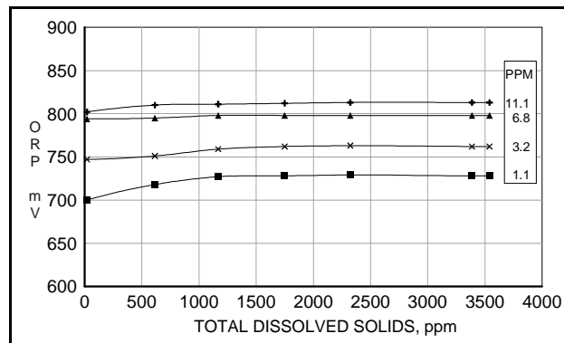
Figure 9 - Effect of TDS on ORP
