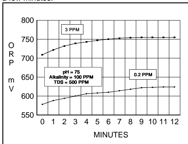
Figure 8 - Time response of ORP Sensor
