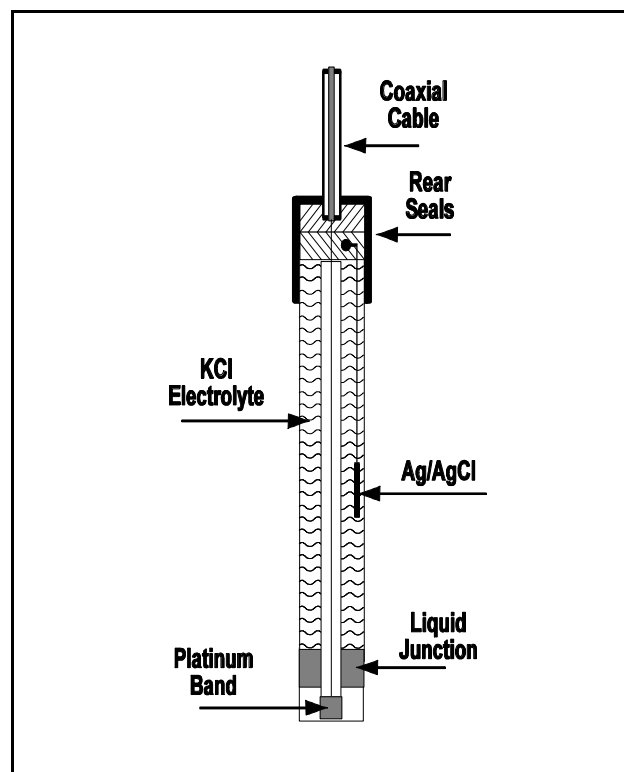
Figure 2 - The ORP Sensor
