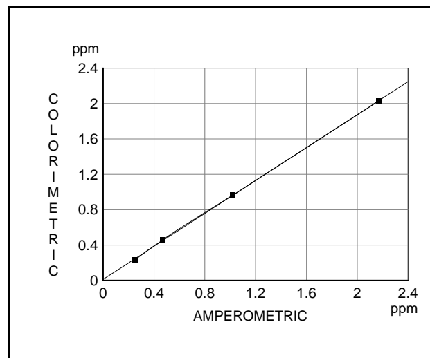
Figure 5 - Comparison of Amperometric Titration and Colorimetric Analysis of Free Chlorine
