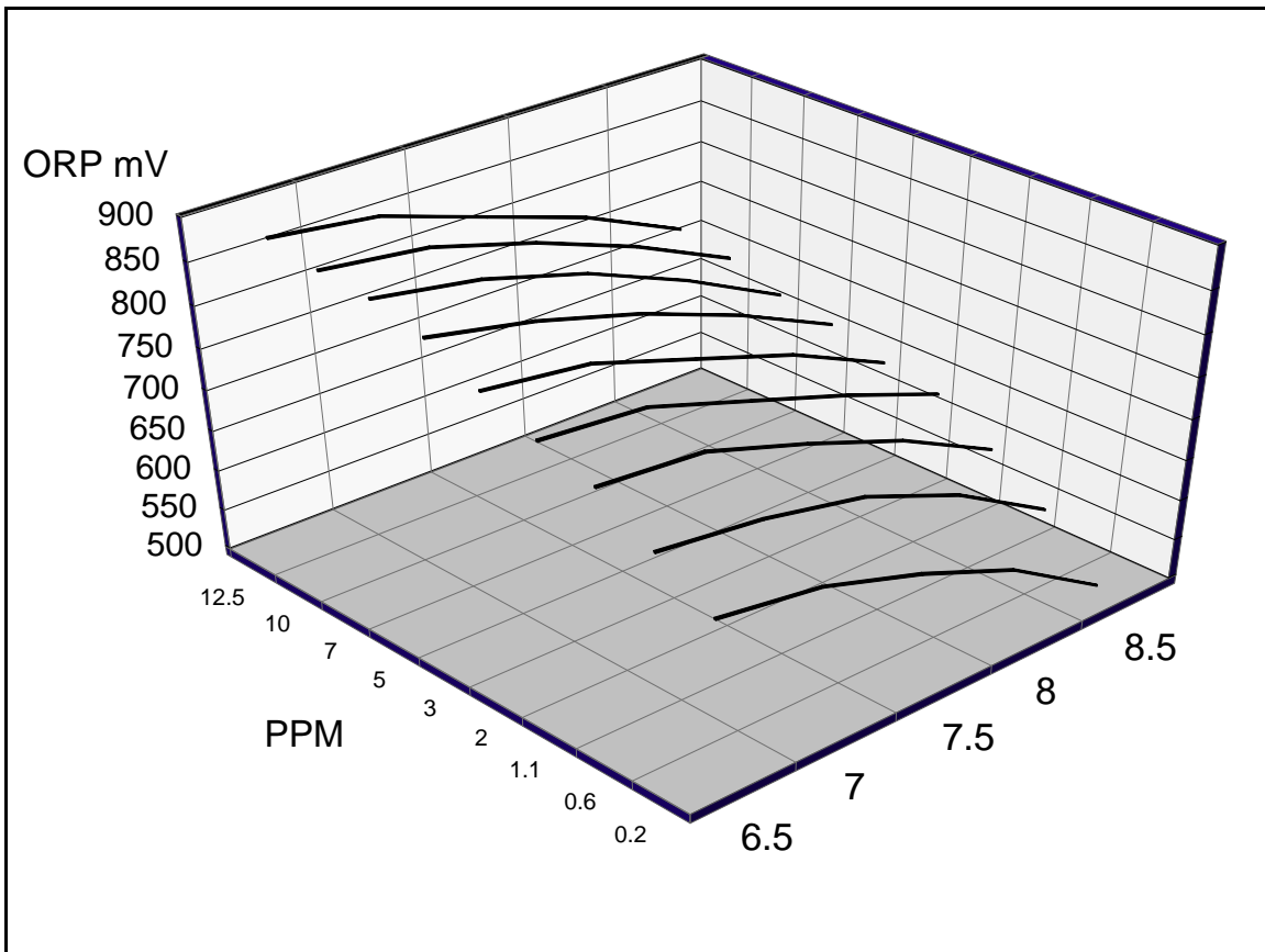
Figure 12 - Variation of ORP with pH and Free Chlorine Concentration
