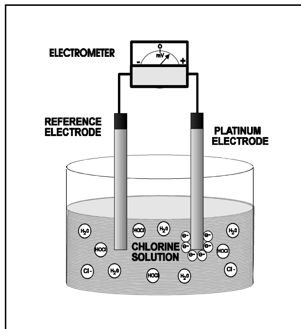
Figure 1 - Schematic of ORP Cell
