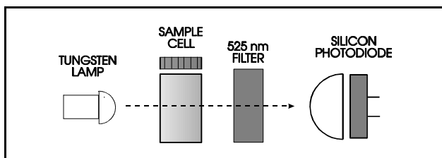
Figure 4 - Colorimetric Analysis of Free Chlorine
