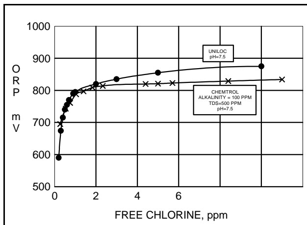
Figure 10 - Comparison of UNILOC and CHEMTROL™ ORP Data at pH 7.5
