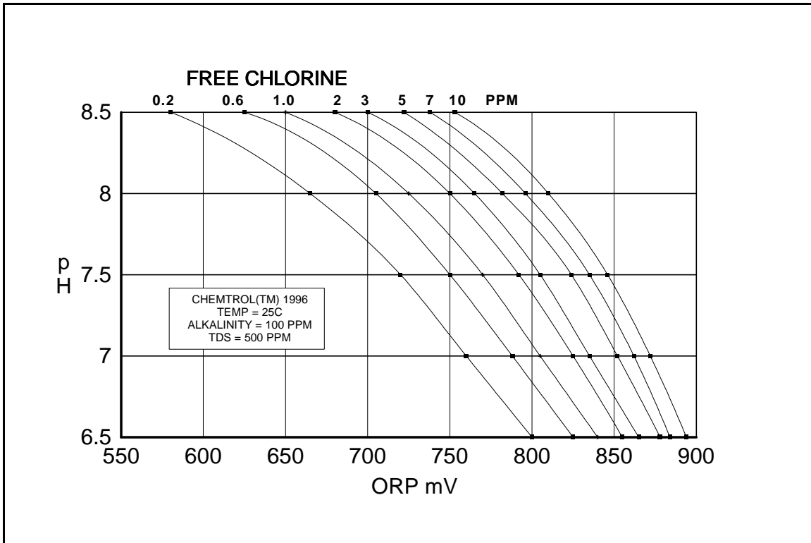
Figure 11 - Variation of ORP of Free Chlorine with pH
