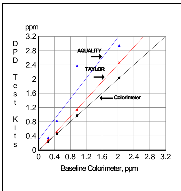
Figure 6 - Comparison of DPD Test Kits
